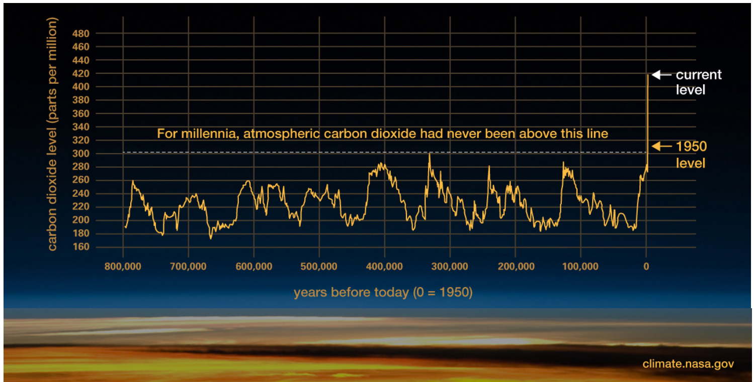
This chart shows carbon dioxide concentrations (vertical axis) over time (horizontal axis) - climate.nasa.gov
